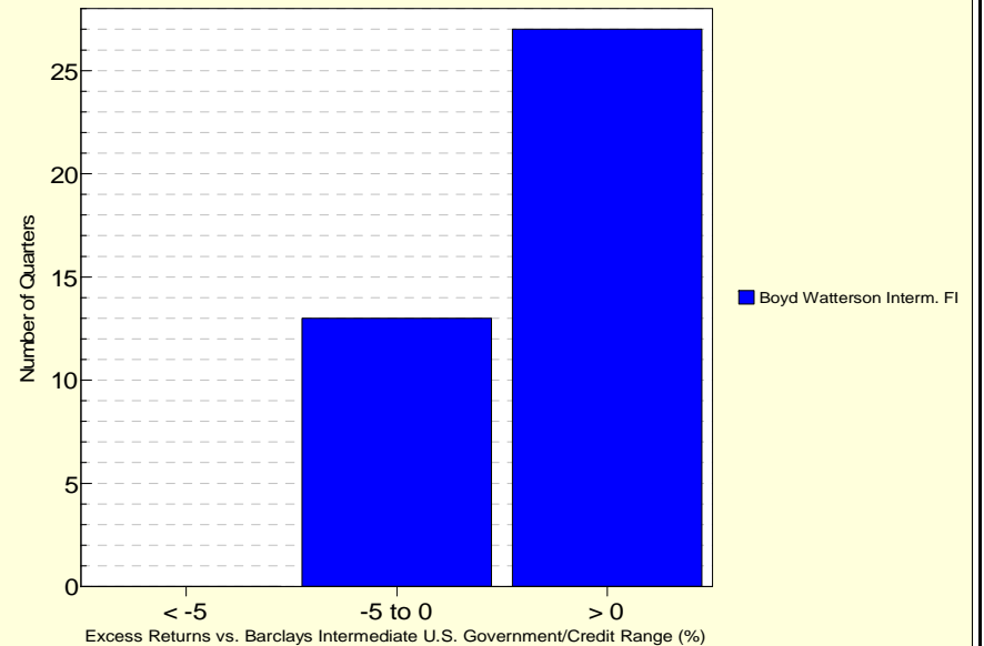
Histogram of Excess Returns vs. Barclays Intermediate U.S. Government/Credit July 2006 - June 2016
